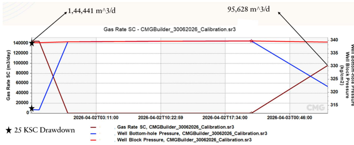
Figure: Simulation Results
