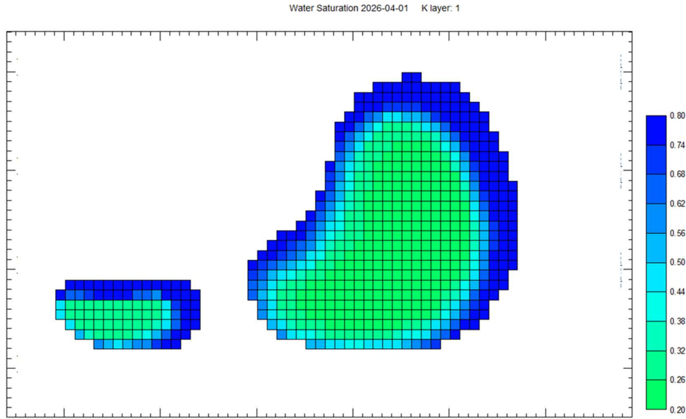
Figure: 2D Model of Saturation
