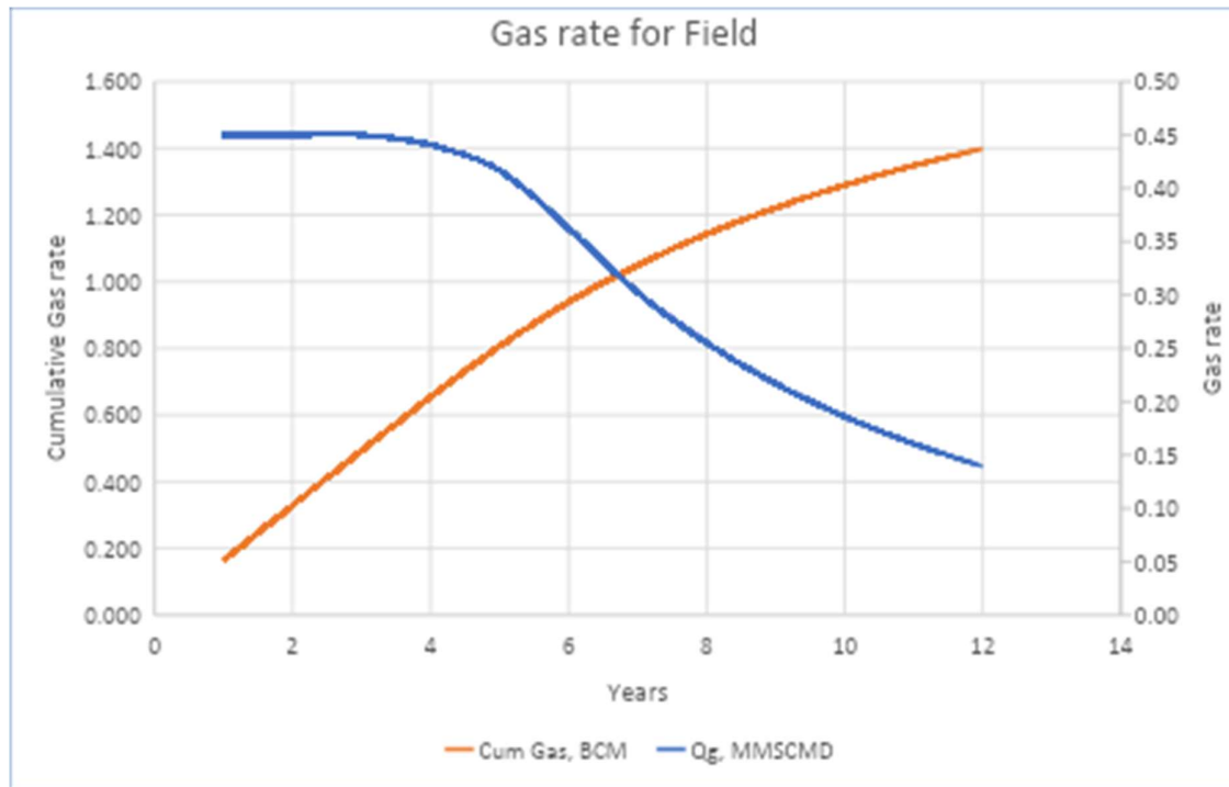
Figure: Production Profile of Total field
