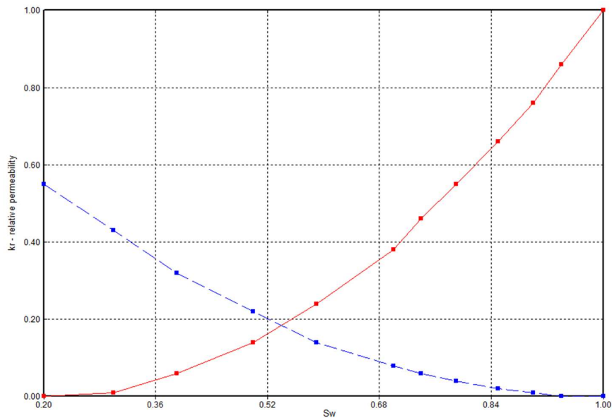
Figure: Relative Permeability Curve
