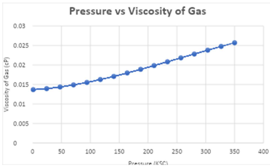
Figure: Gas Viscosity with Pressure
