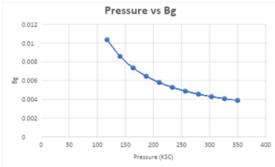
Figure: Pressure vs Bg Plot
