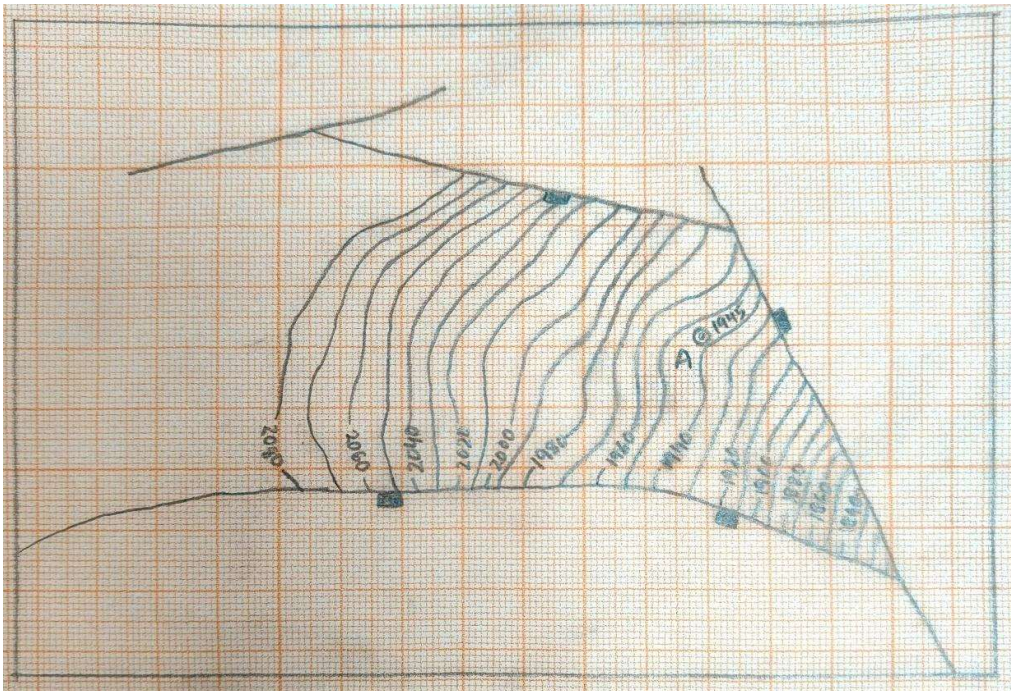
Figure: Structure Contour Map
