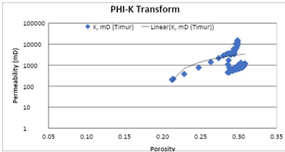
Figure: Phi -K Transform Plot
