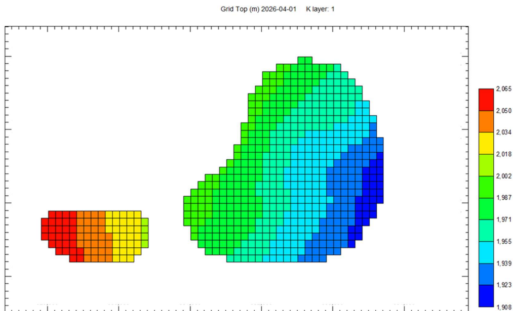
Figure: 2D Model of Grid Top
