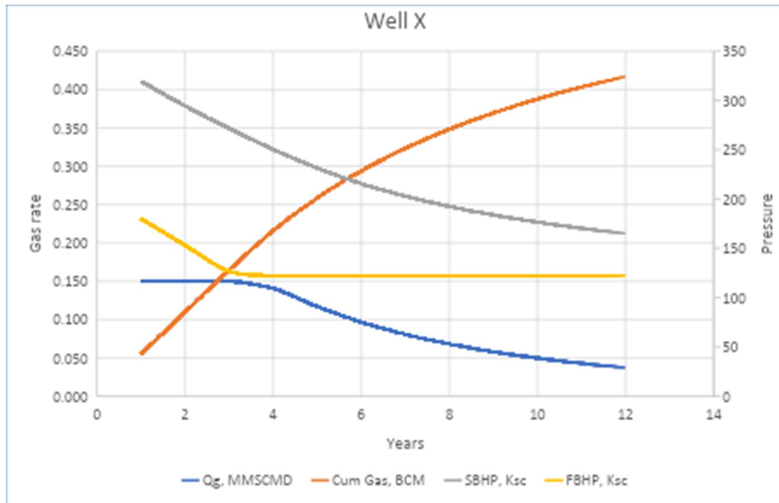
Figure: Production Profile of Well X
