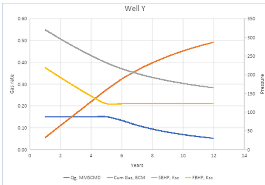
Figure 41: Production Profile of Well Y
