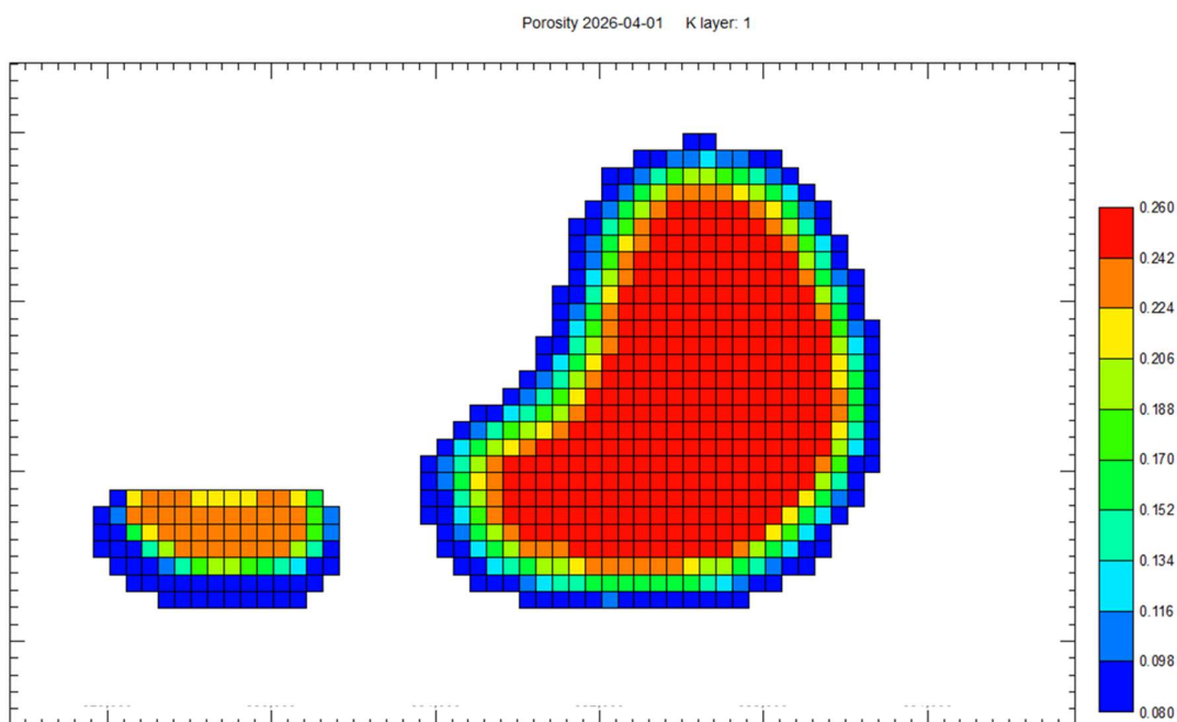
Figure: 2D Model of Porosity
