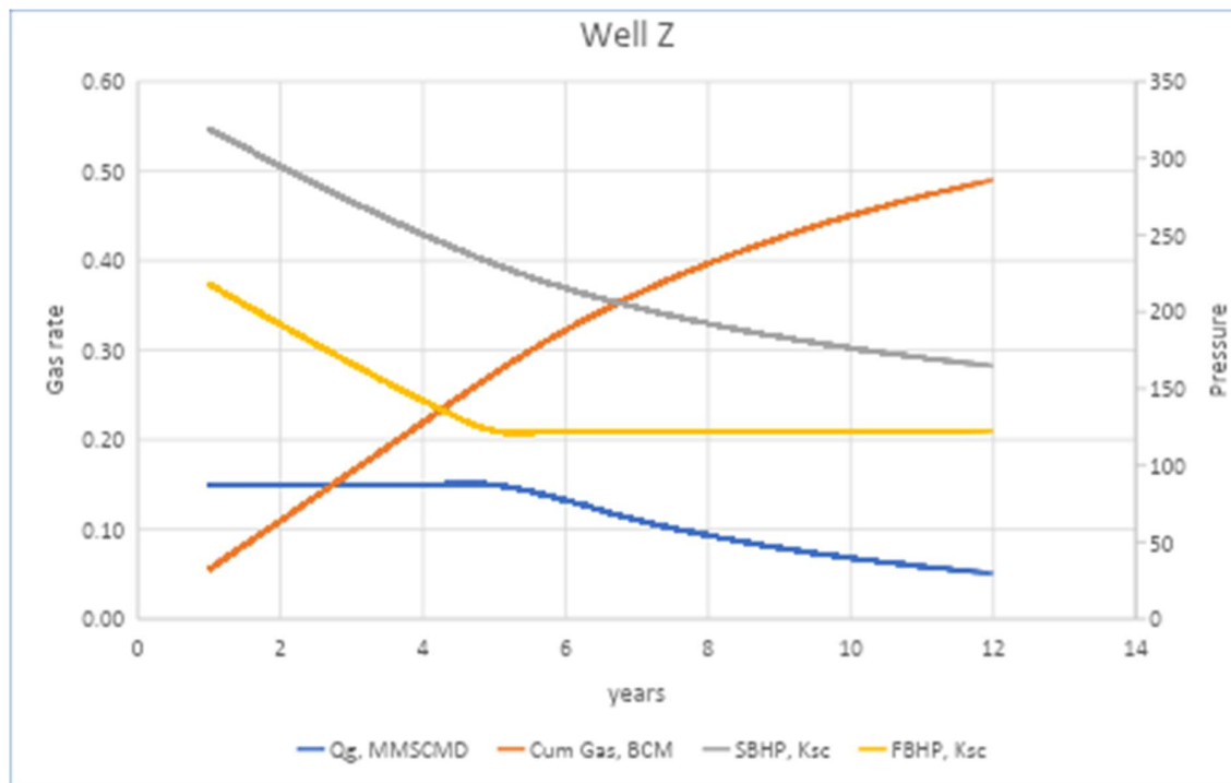
Figure: Production Profile of Well Z
