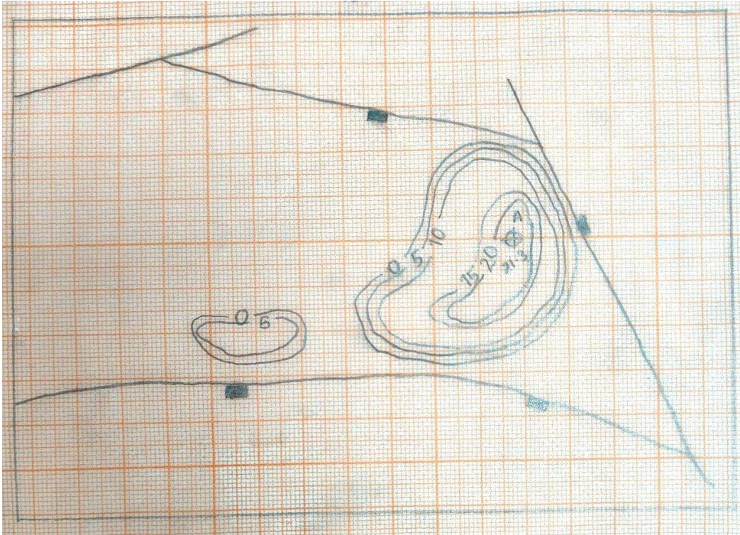
Figure: Isopay Map
